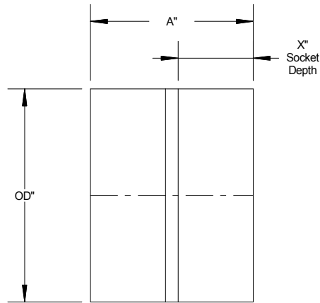
Sleeve Coupling
