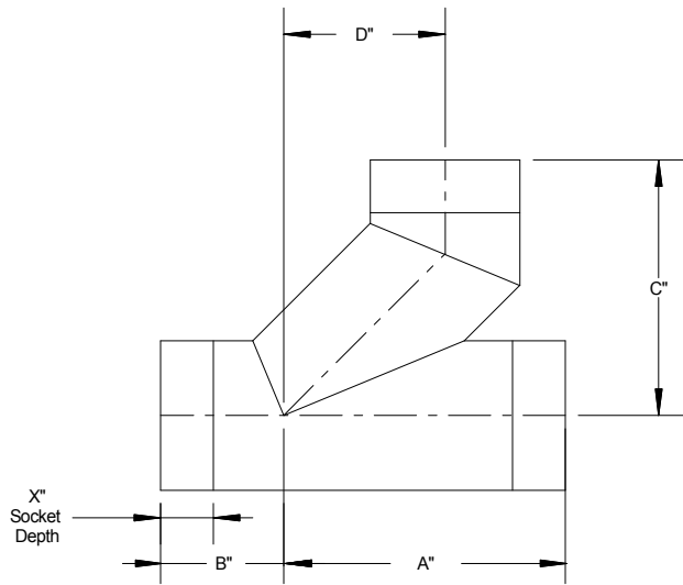
45 deg Combination Lateral
