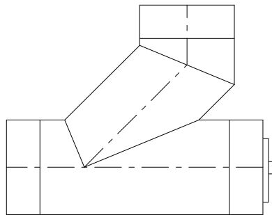
45 deg Combination Lateral with Cleanout Position 2
