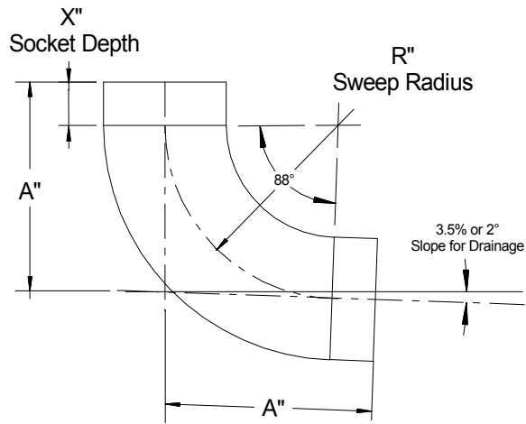
88 deg Ell Note: Other Slopes Available
