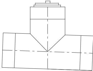
2 deg Offset Tee with Cleanout Position 3 Note: Other Slopes Available
