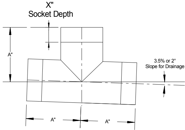
2 deg Offset Tee Note: Other Slopes Available
