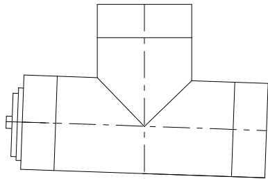
2 deg Offset Tee with Cleanout Position 2 Note: Other Slopes Available
